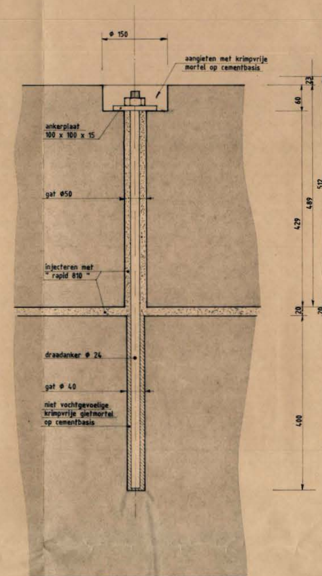
DETAIL 1 BEVESTIGINGS ANKER
